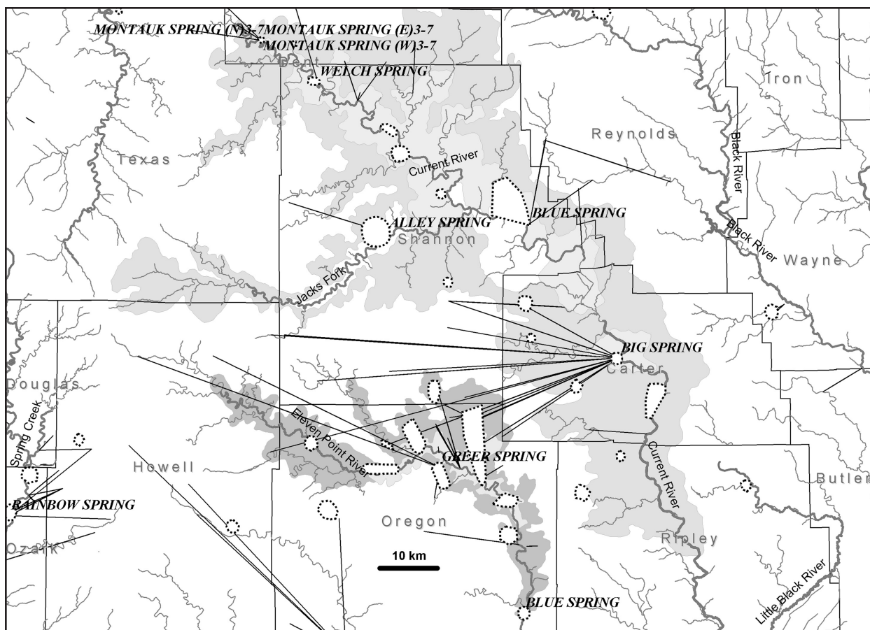
Figure 5. The Missouri Cave Focus Areas include magnitude 1 springs, such as this part of southeastern Missouri. Dye traces are shown as thin lines and cave focus areas as dotted outlines. Much of the flow of the Eleven Point River is pirated underground to Big Spring and the Current River.
